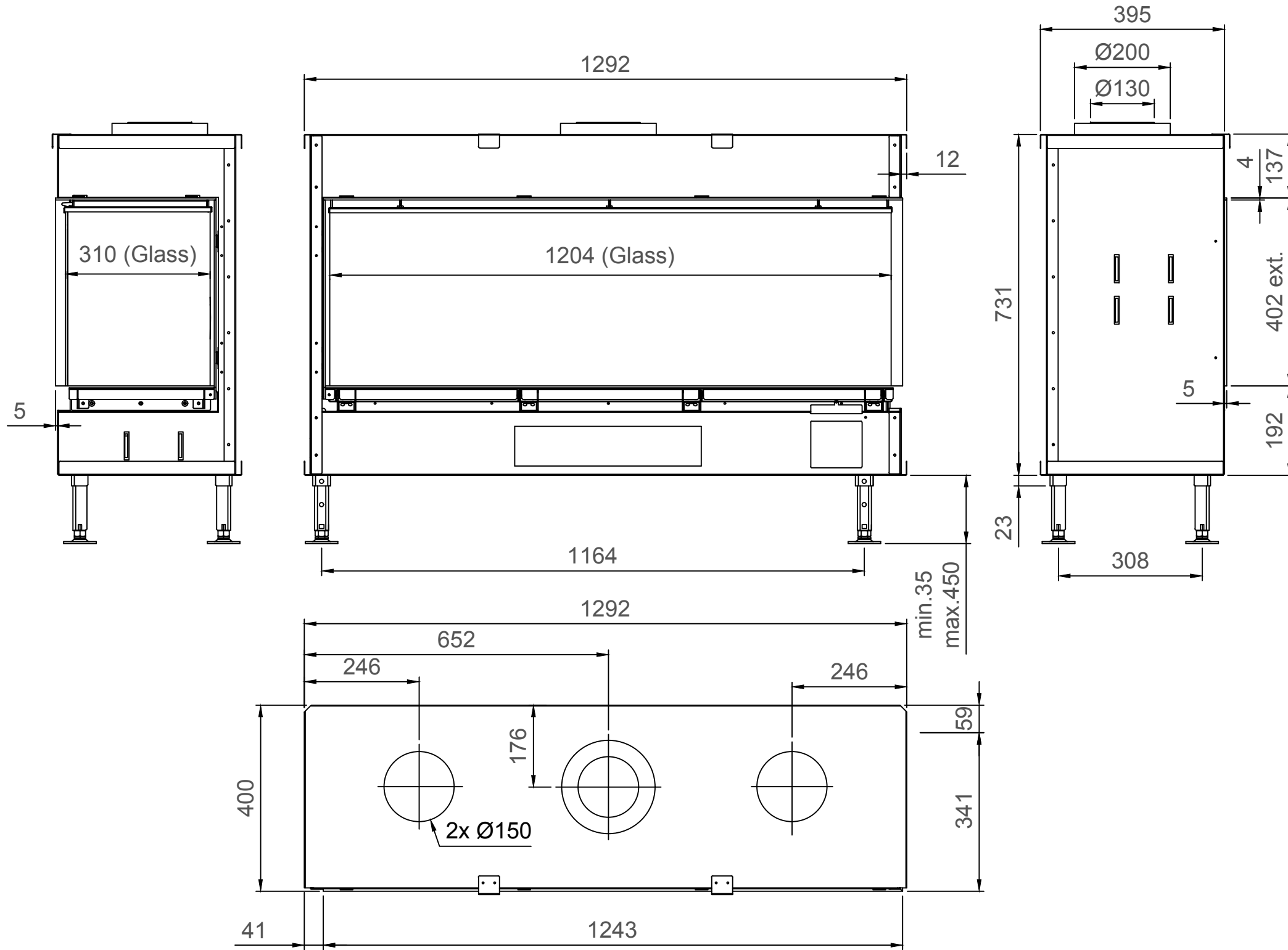
Luna Diamond 1300CR Gas/Gaz - Type 1 - Coverframe
