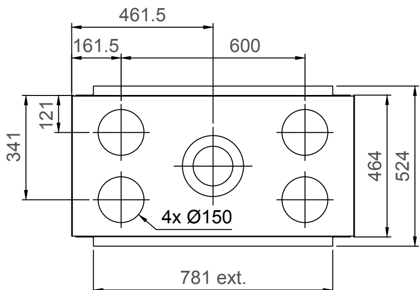
True Vision 850DVL - TV - Type 3 - 30mm
