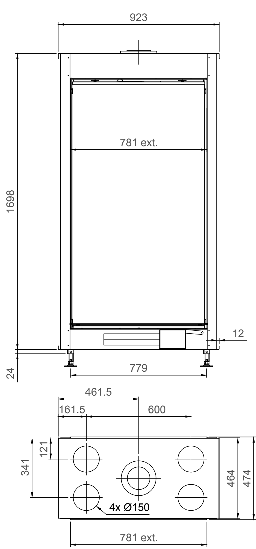
True Vision 850DVL - TV - Type 1 - Coverframe
