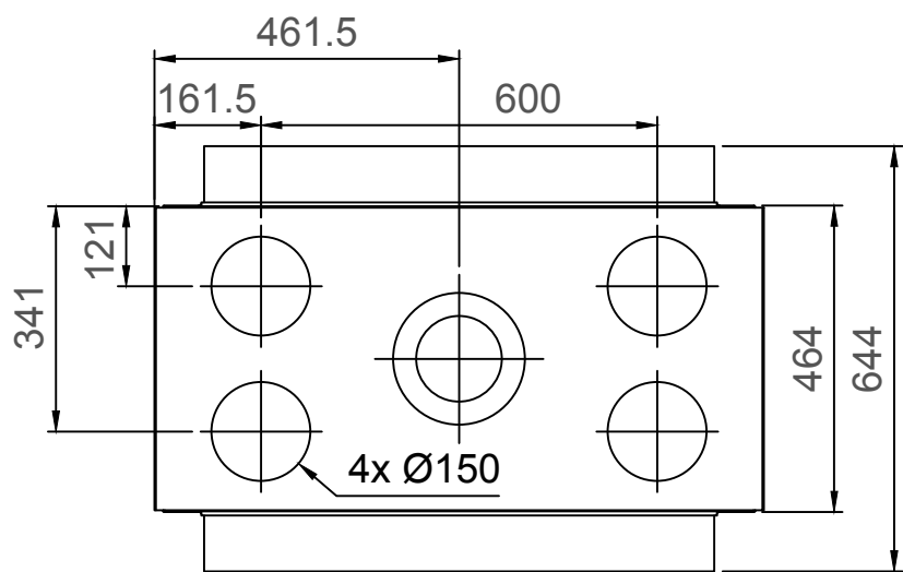
True Vision 850DVL - TV - Type 2 - 90mm
