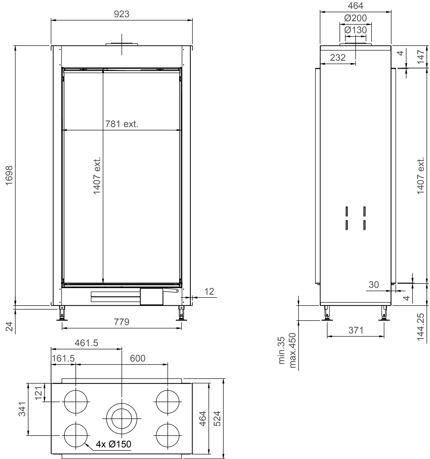
True Vision 850DVL - TV - Type 4 - 30mm
