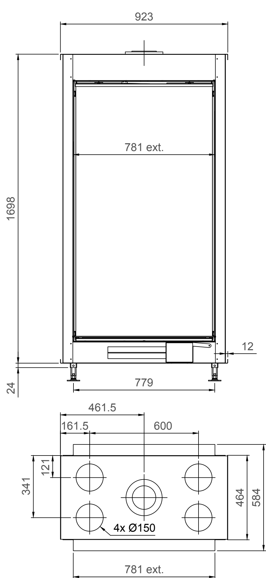
True Vision 850DVL - TV - Type 3 - 60mm
