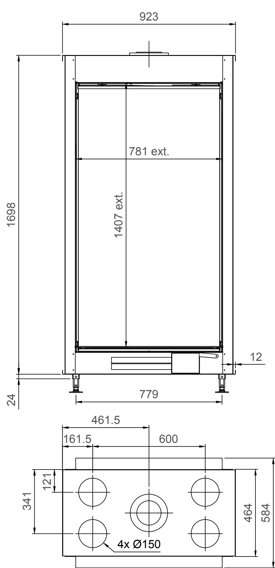
True Vision 850DVL - TV - Type 4 - 60mm
