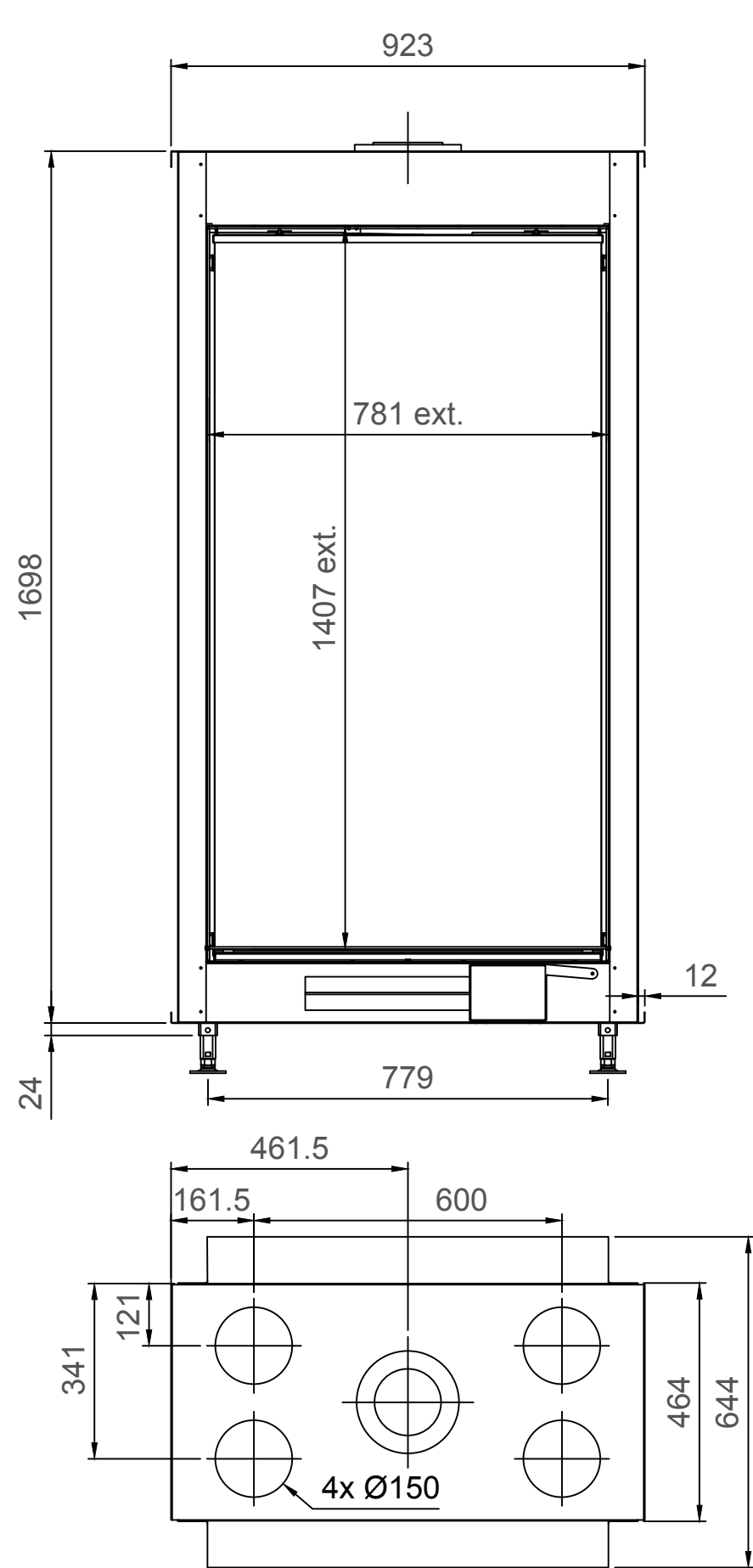
True Vision 850DVL - TV - Type 4 - 90mm
