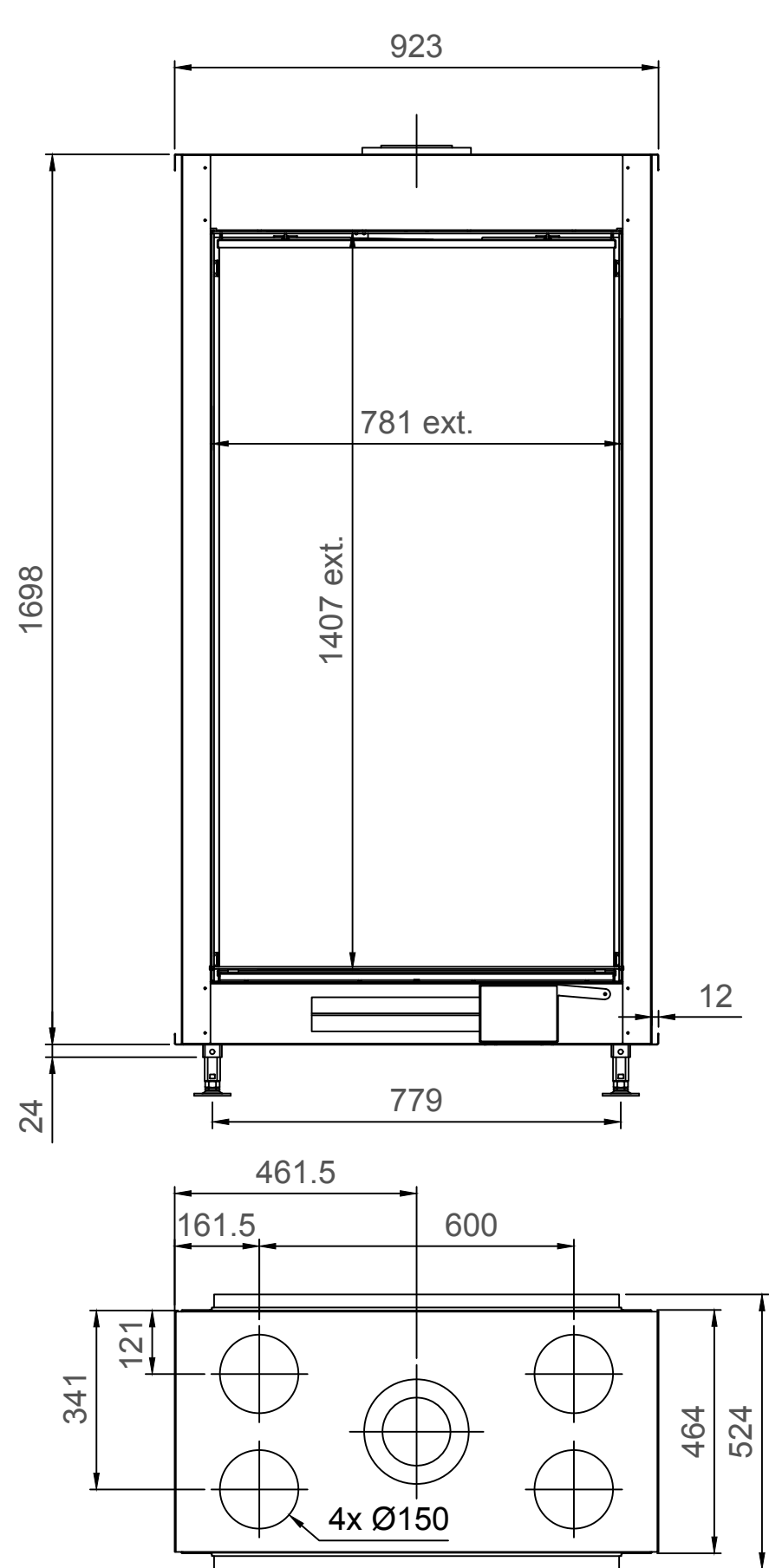
True Vision 850DVL - TV - Type 2 - 30mm
