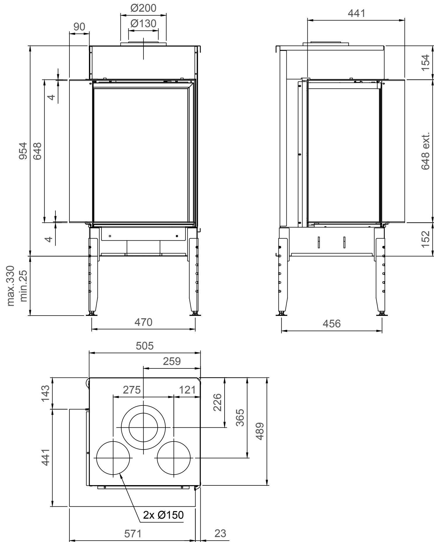
True Vision 550CL - Type 4 - 90mm
