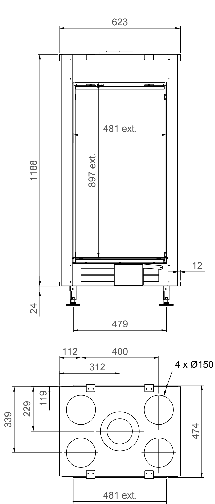
True Vision 550DV - Type 1 - Coverframe
