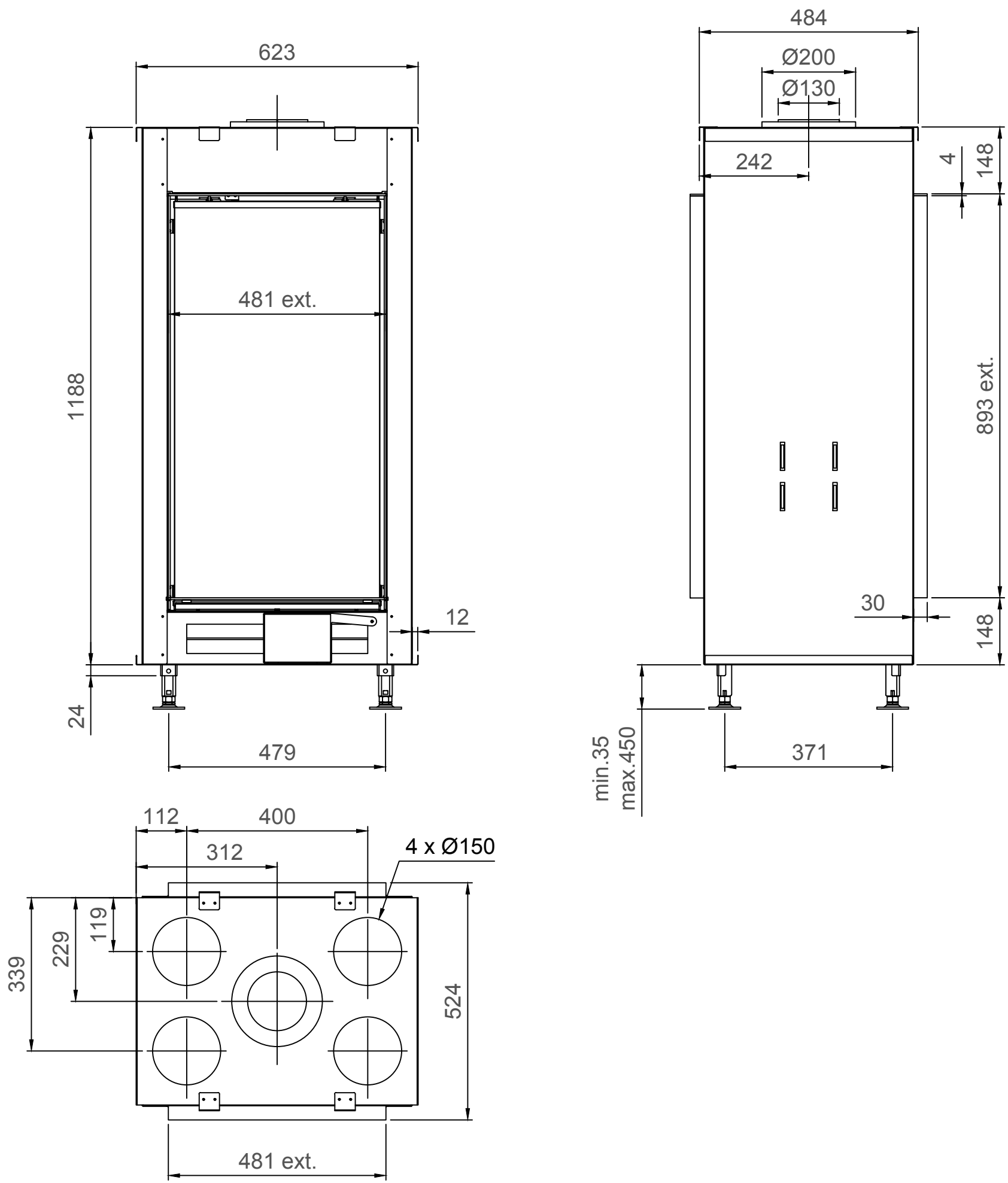
True Vision 550DV - Type 3 - 30mm
