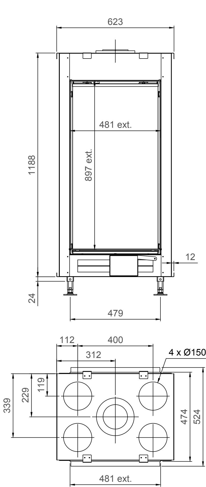
True Vision 550DV - Type 2 - 30mm
